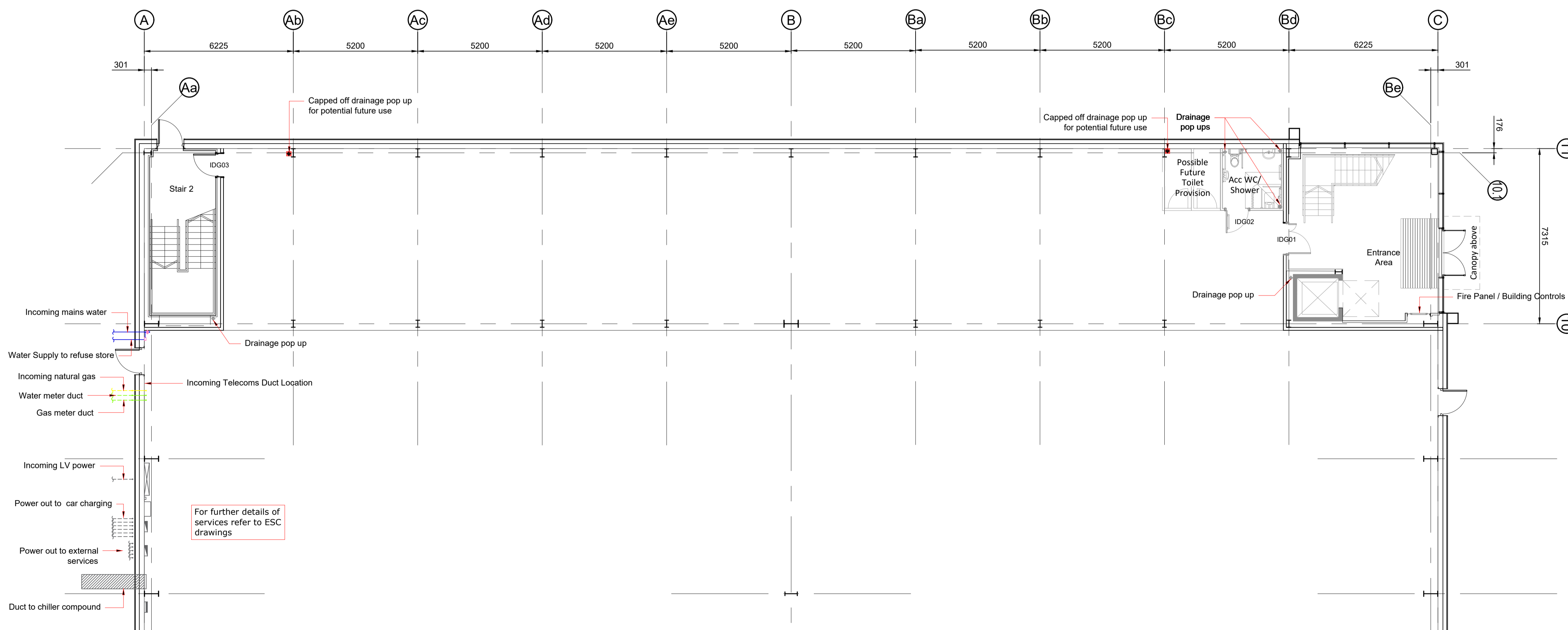
Ground Floor Office Plan Scale 1:100
